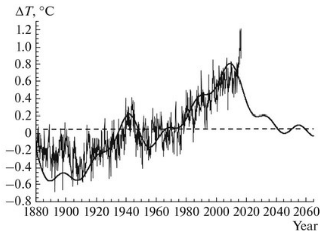
Figure 2.3.1.1.3 Changes in global near-surface air temperature from 1880–2015 and forecast after 2015
